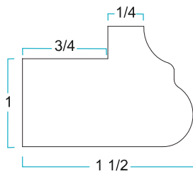
Light Rail Molding/Angle Light Rail Molding
